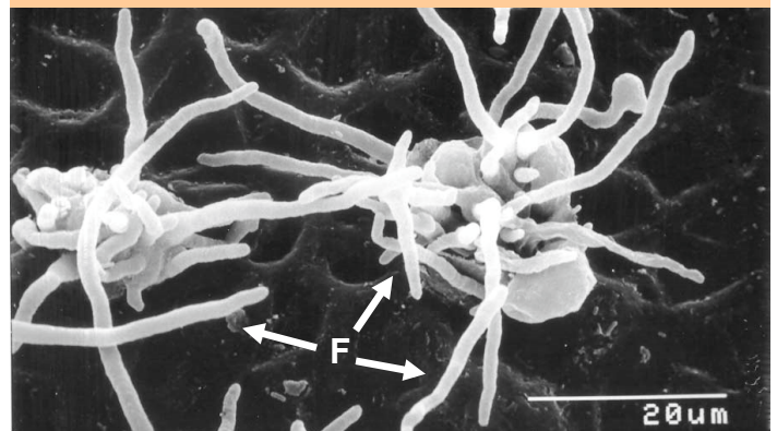
Once infection is established, fungal strands (F) grow out of the host to form more sporangia.
