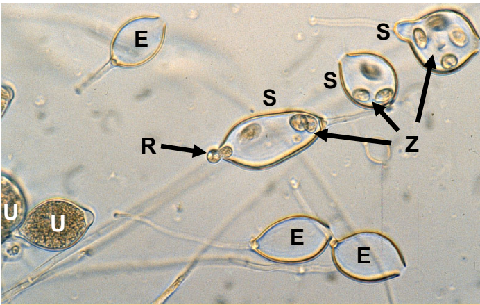
Spread of Phytophthora capsici in water. When immersed in water, the contents of undifferentiated sporangia (U) form swimming spores (zoospores, Z) inside the sporangia (S). The zoospores are released (R) into the water, leaving empty sporangia (E).
