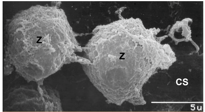
Zoospores (Z) attach to a cucumber surface (CS) using a sticky matrix.
