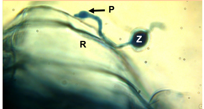
A zoospore (Z) that has germinated on and penetrated (P) into a pepper root (R).
